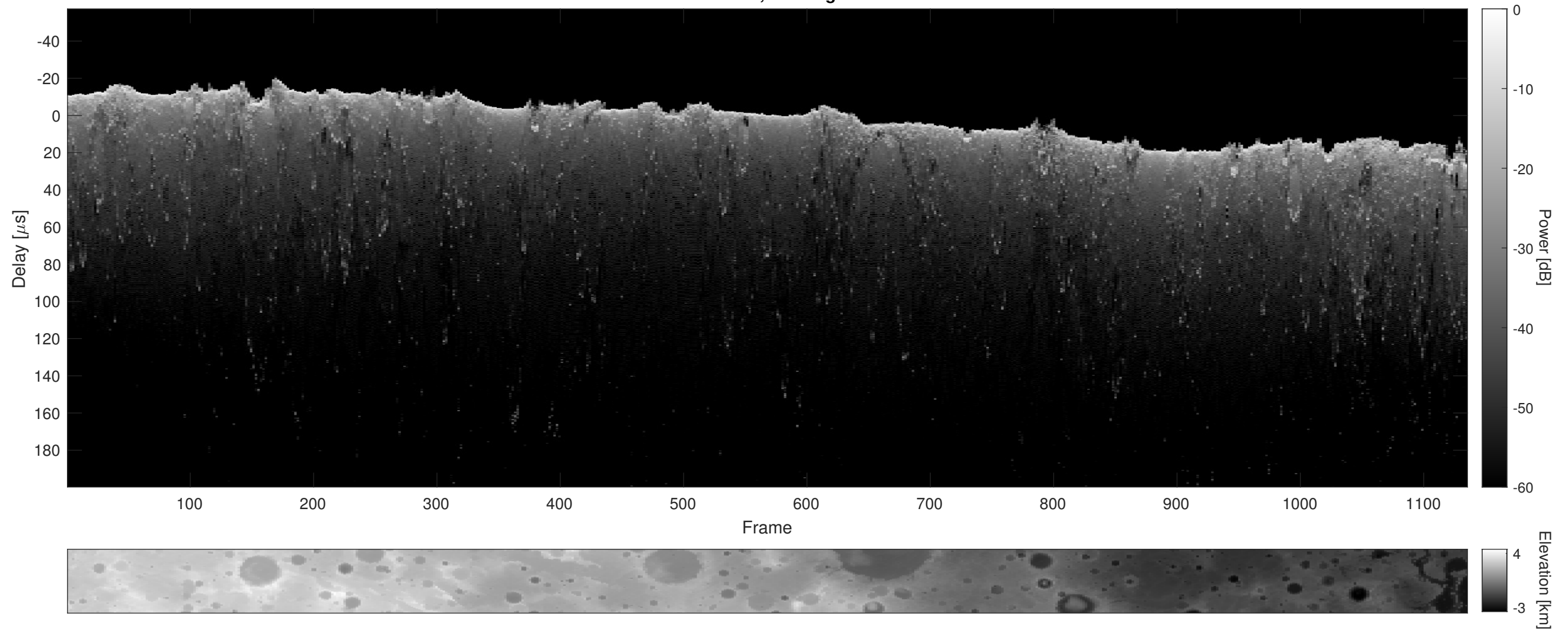
Orbit 20841, Cluttergram
