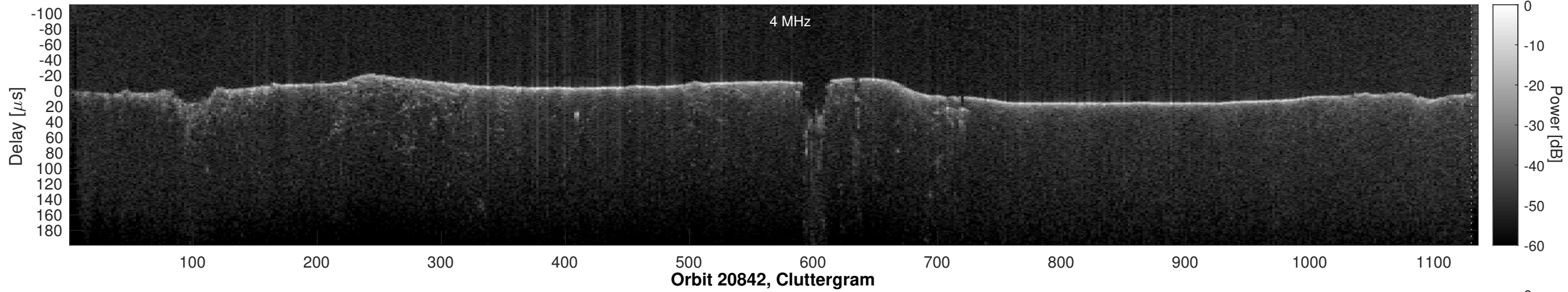
Orbit 20842, Window, Channel 1, Optimized
