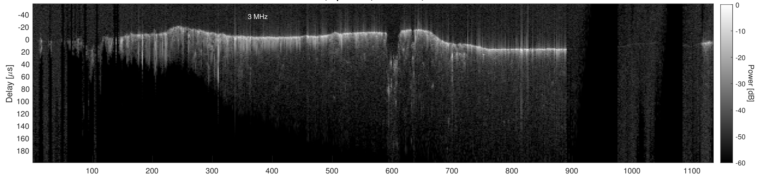
Orbit 20842, Cluttergram
