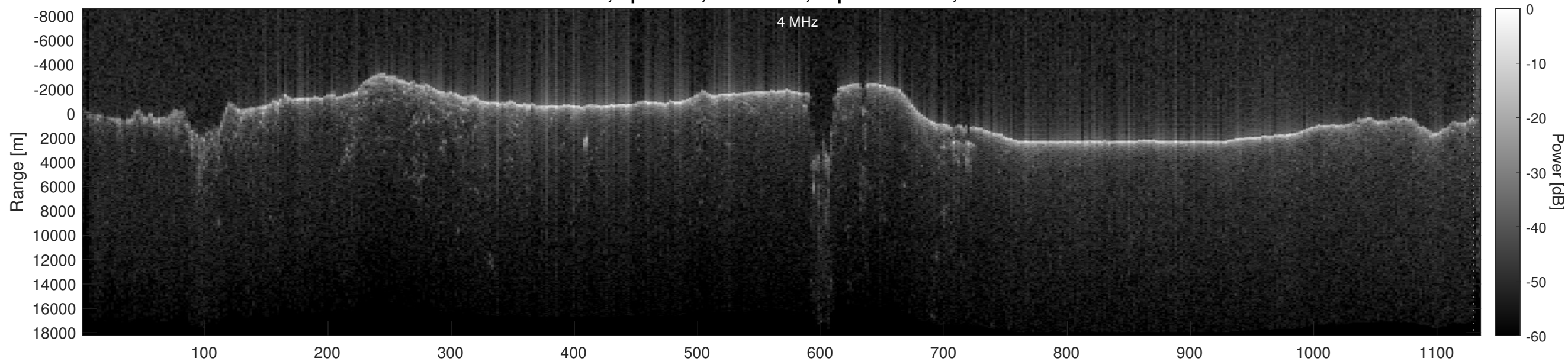
Orbit 20842, Optimized, No Window, Depth-Corrected, Channel 2
