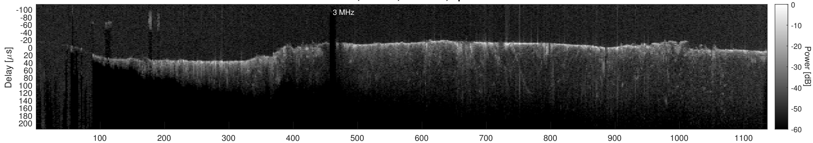
Orbit 20844, Cluttergram
