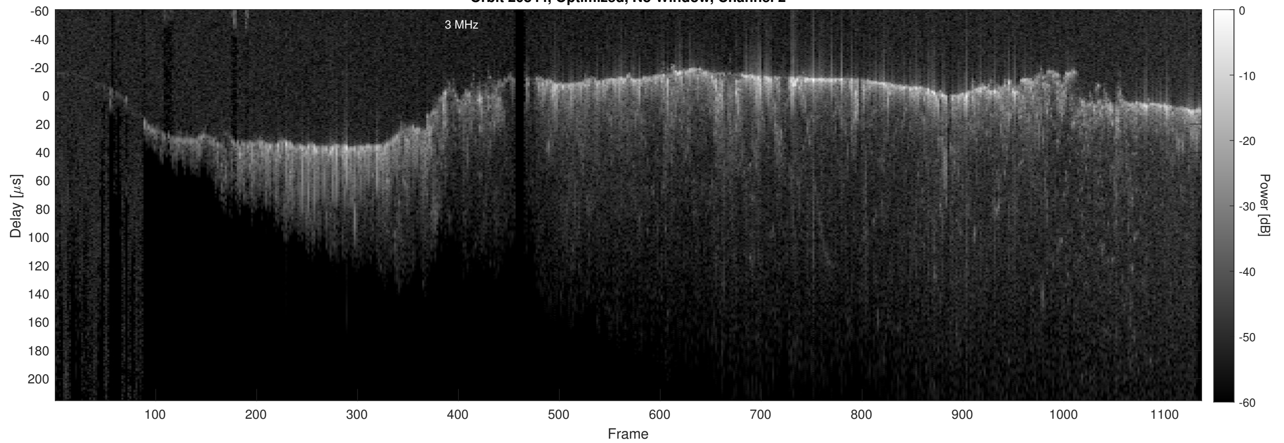
Orbit 20844, Optimized, No Window, Channel 2
