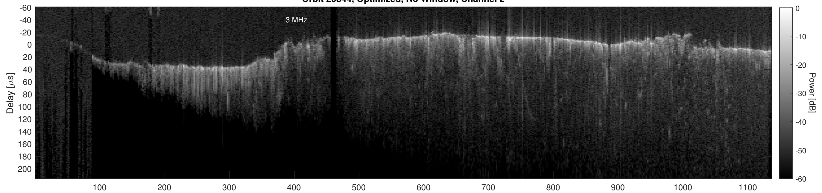
Orbit 20844, Cluttergram
