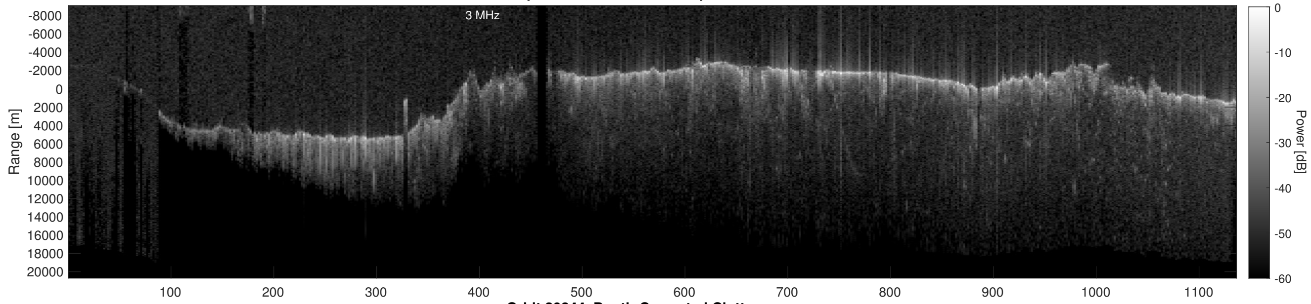
Orbit 20844, Depth-Corrected Cluttergram
