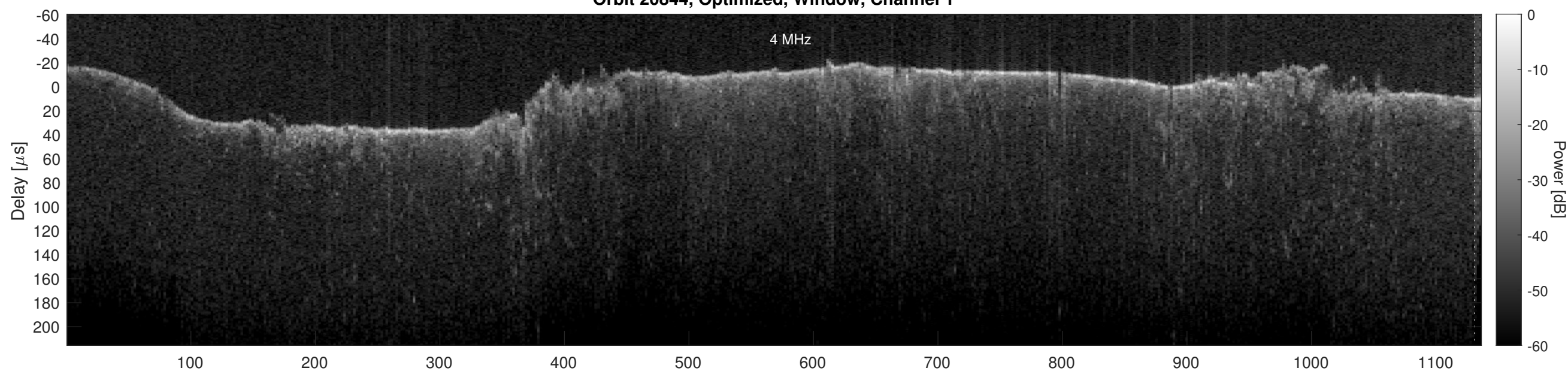
Orbit 20844, Optimized, Window, Channel 2
