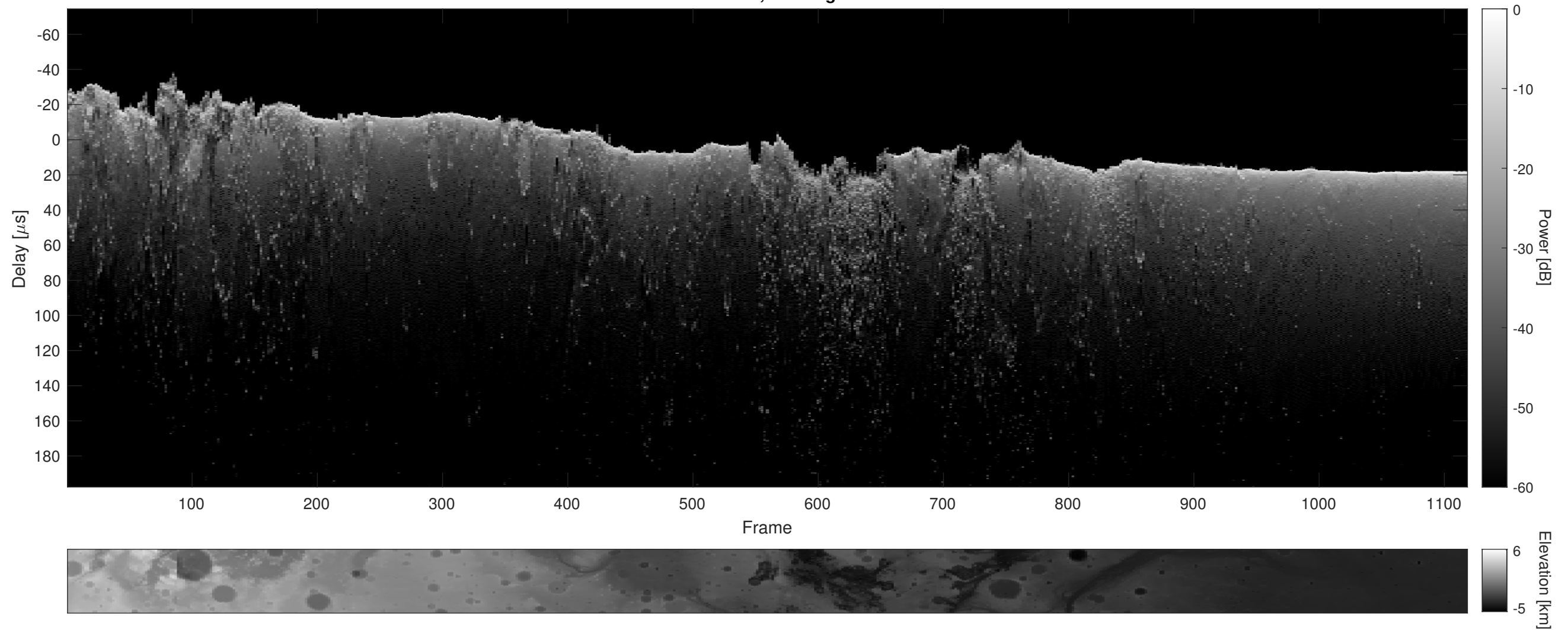
Orbit 20845, Cluttergram
