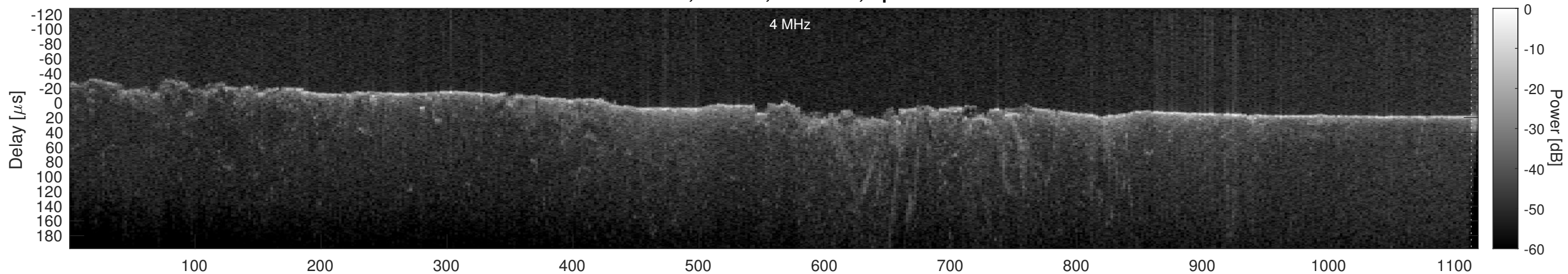
Orbit 20845, Cluttergram
