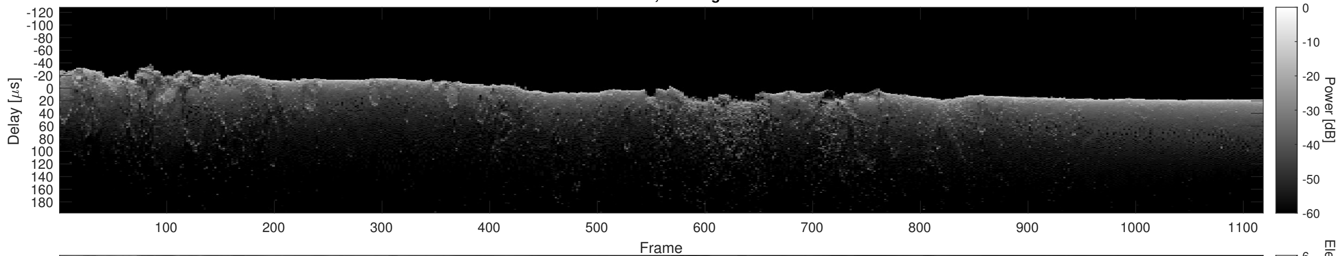
Orbit 20845, Cluttergram
