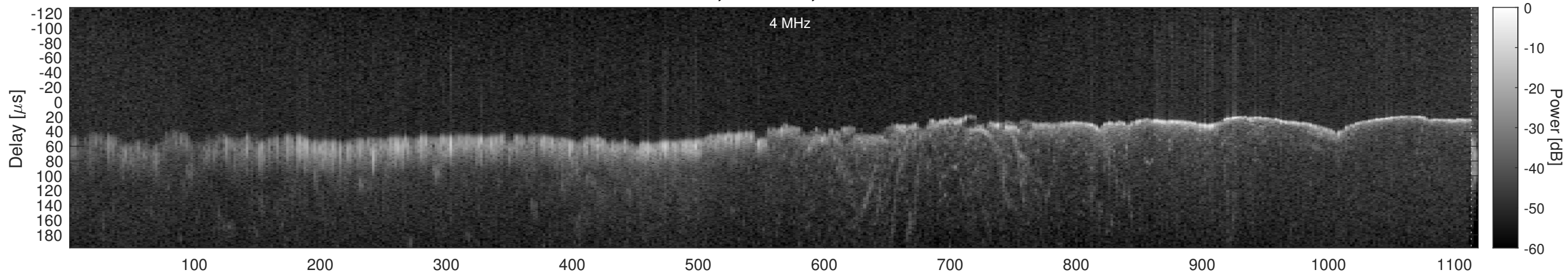
Orbit 20845, Window, Channel 1, Chapman
