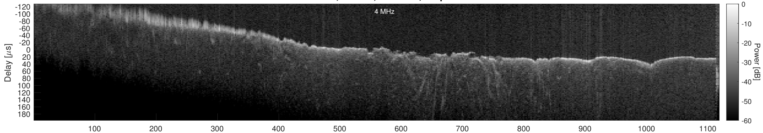
Orbit 20845, Window, Channel 1, Optimized
