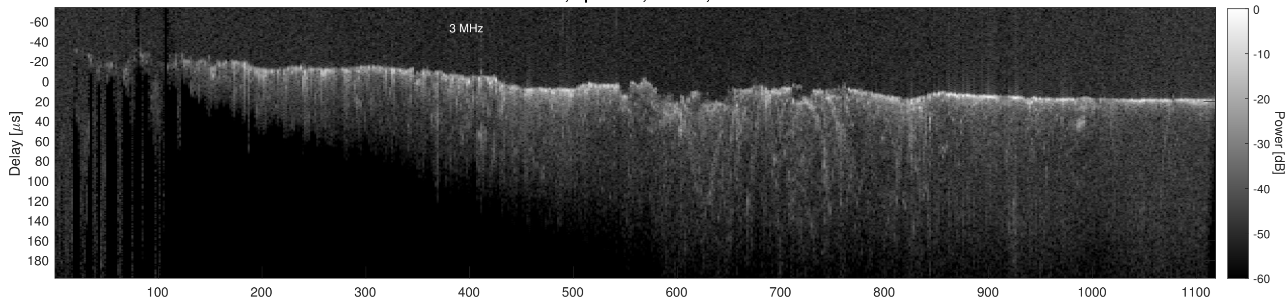
Orbit 20845, Cluttergram
