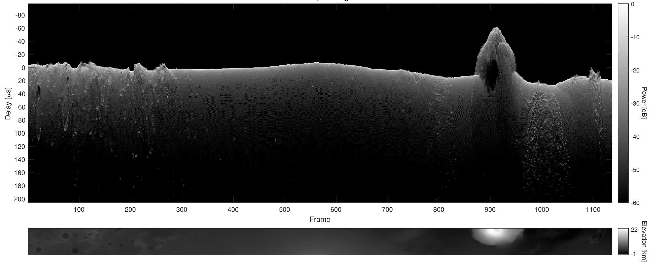
Orbit 20846, Cluttergram
