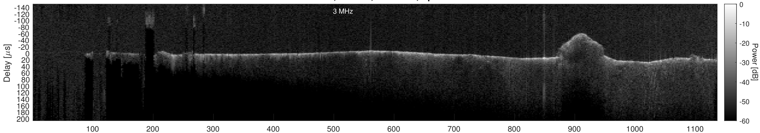
Orbit 20846, Cluttergram
