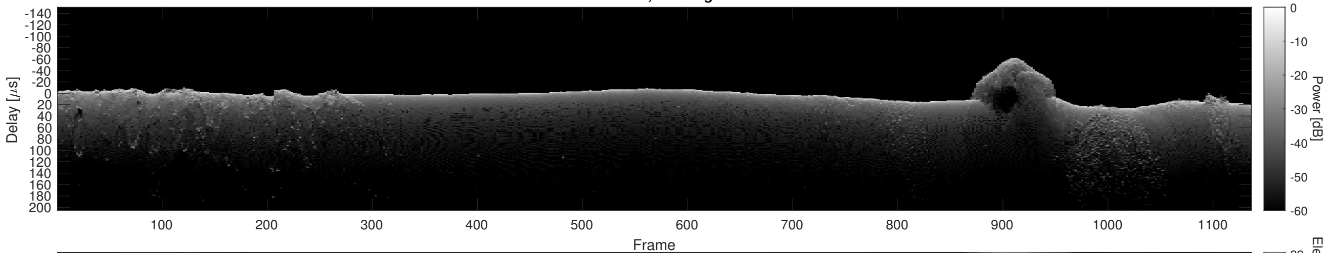
Orbit 20846, Cluttergram
