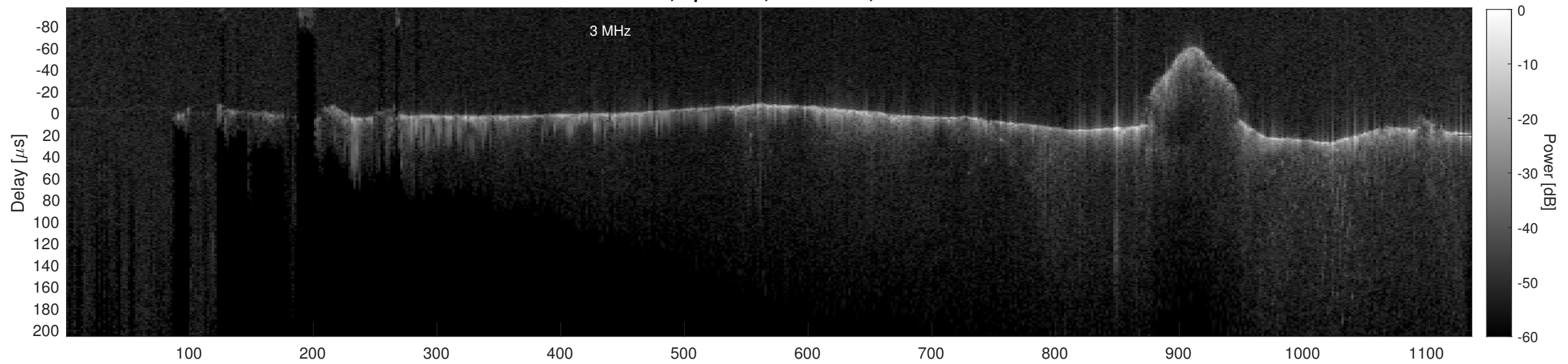
Orbit 20846, Cluttergram
