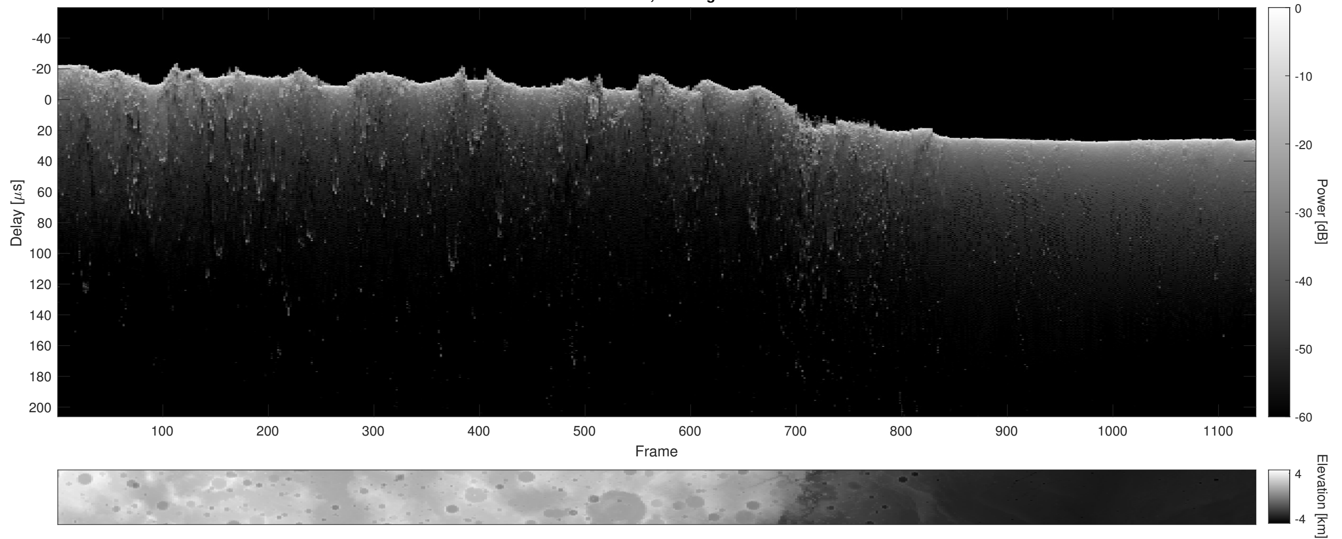
Orbit 20847, Cluttergram
