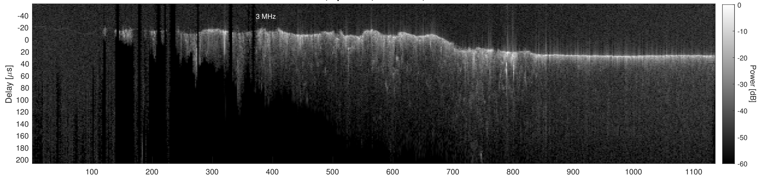
Orbit 20847, Cluttergram
