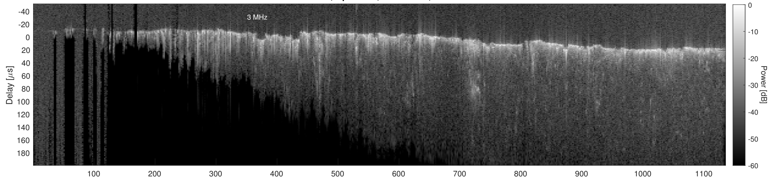
Orbit 20848, Cluttergram
