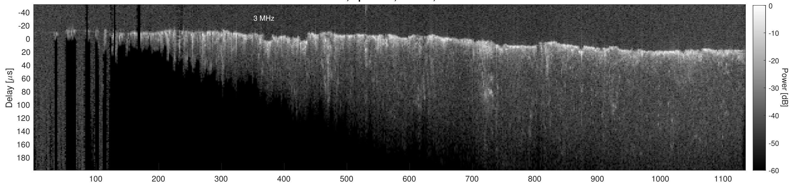
Orbit 20848, Cluttergram
