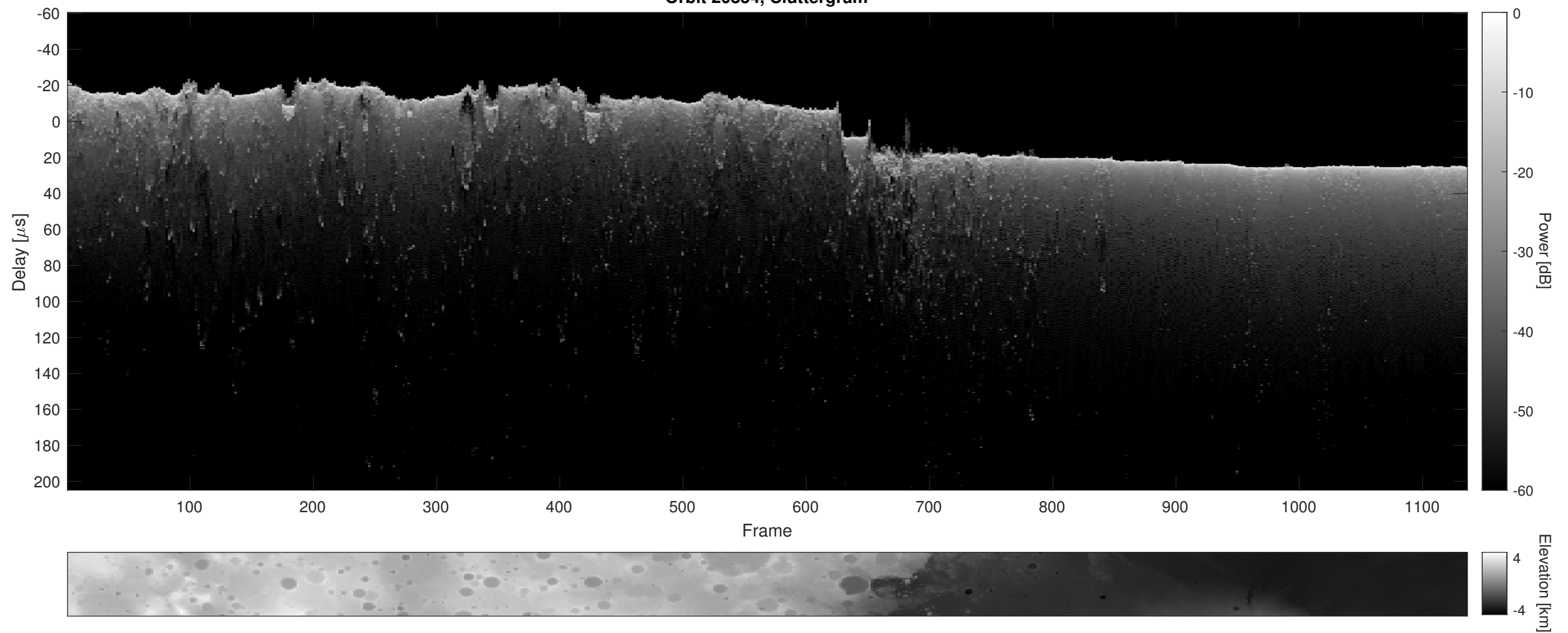
Orbit 20854, Cluttergram
