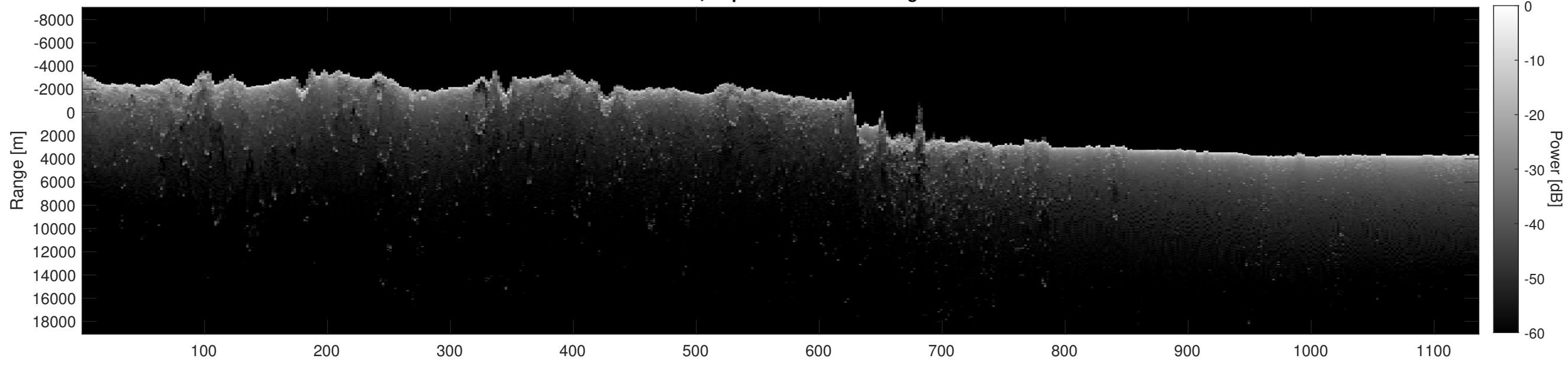
Orbit 20854, Depth-Corrected Cluttergram
