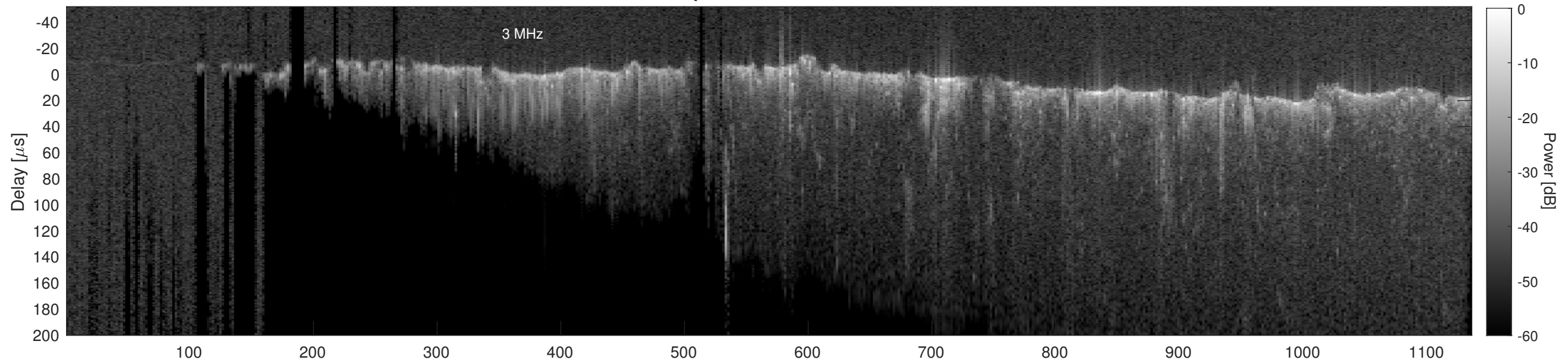
Orbit 20855, Cluttergram
