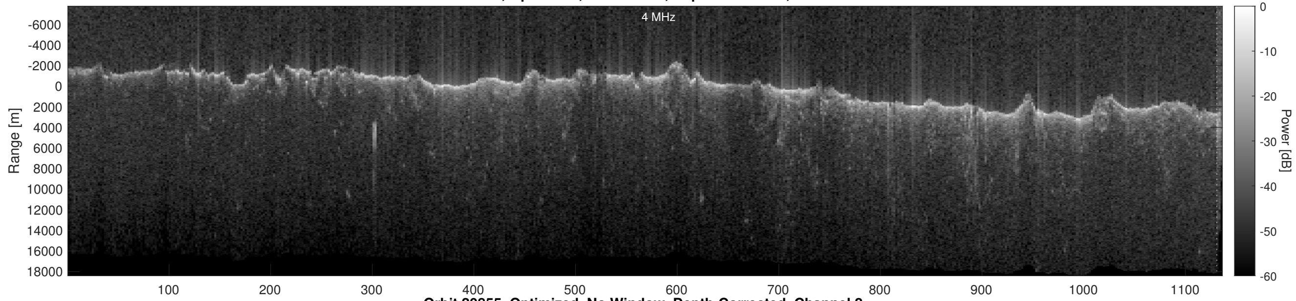
Orbit 20855, Optimized, No Window, Depth-Corrected, Channel 2
