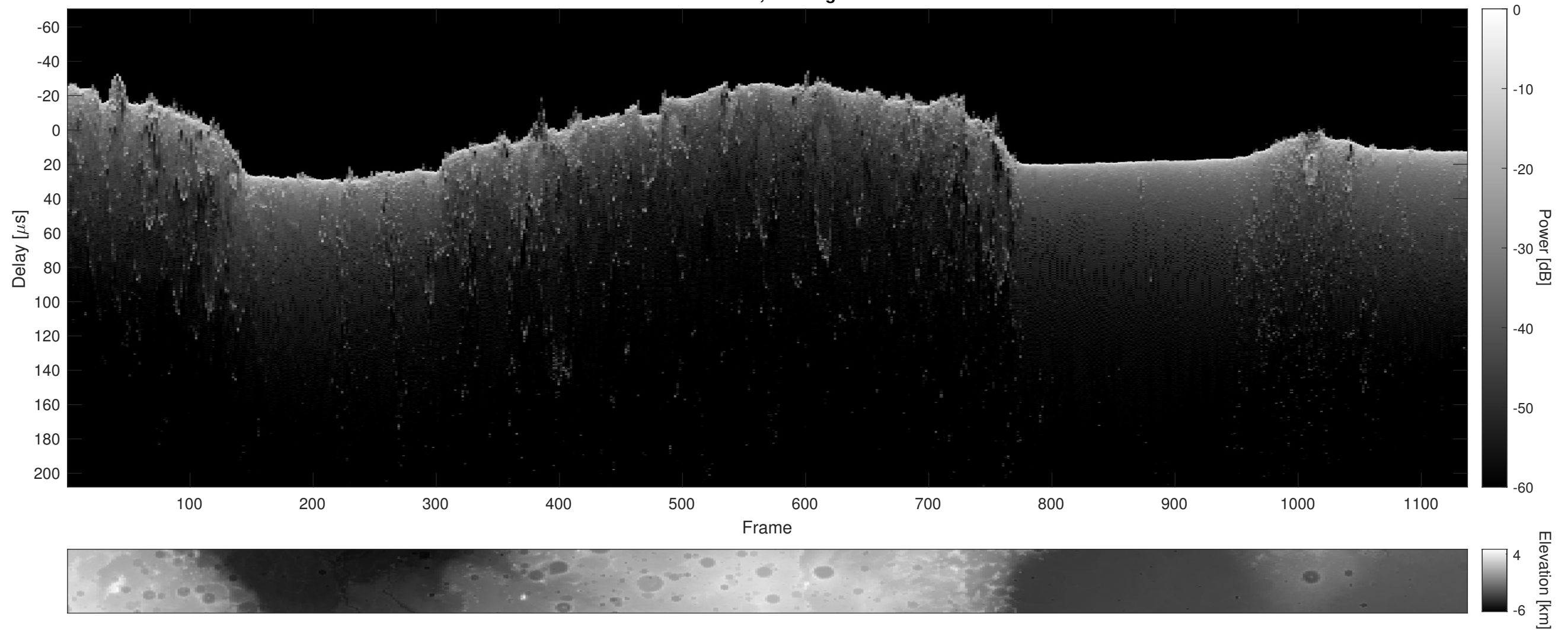
Orbit 20858, Cluttergram
