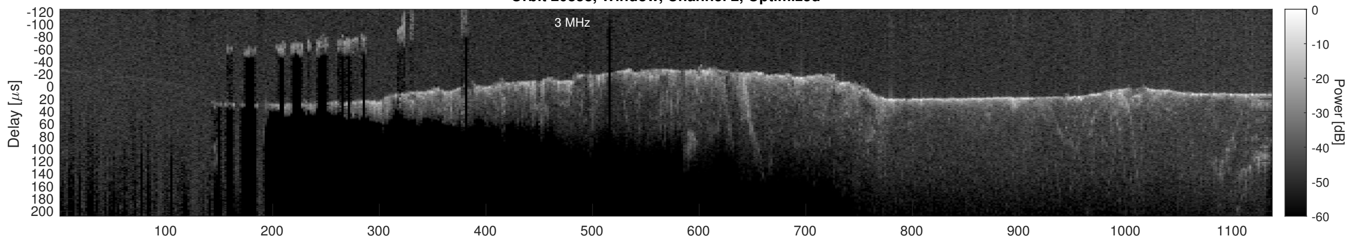
Orbit 20858, Cluttergram
