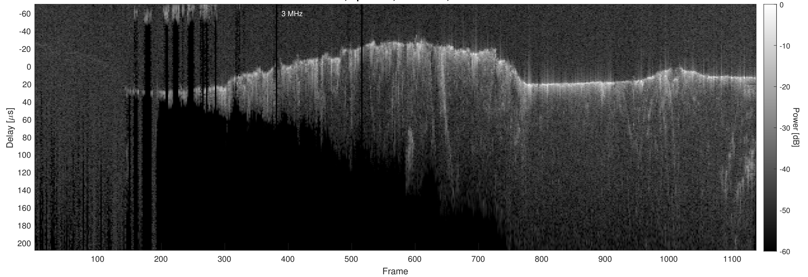
Orbit 20858, Optimized, No Window, Channel 2
