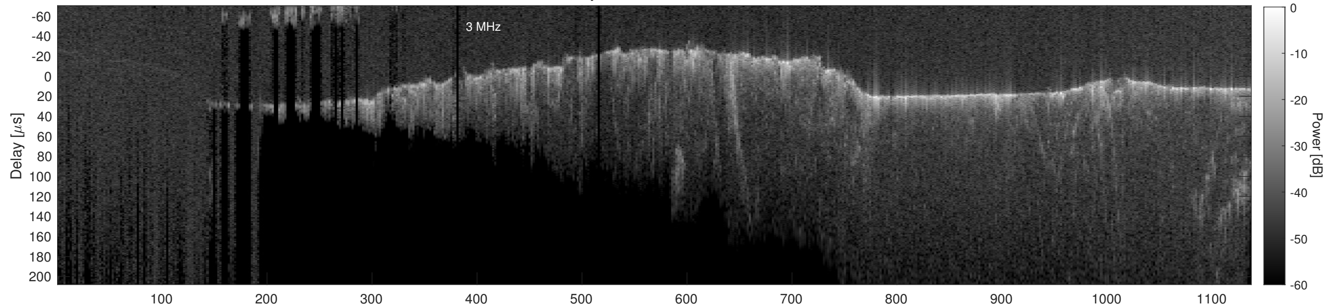
Orbit 20858, Cluttergram
