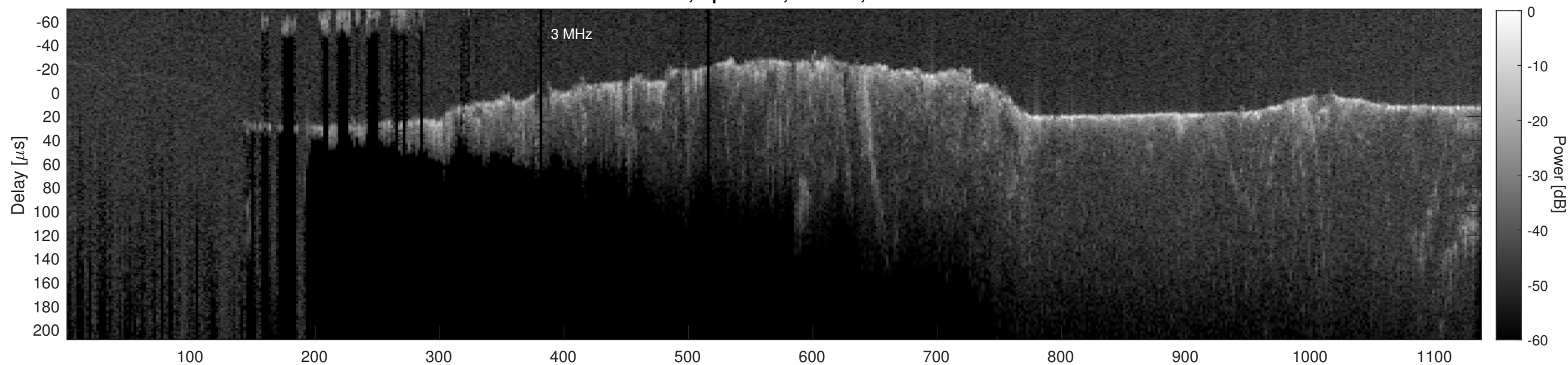
Orbit 20858, Cluttergram
