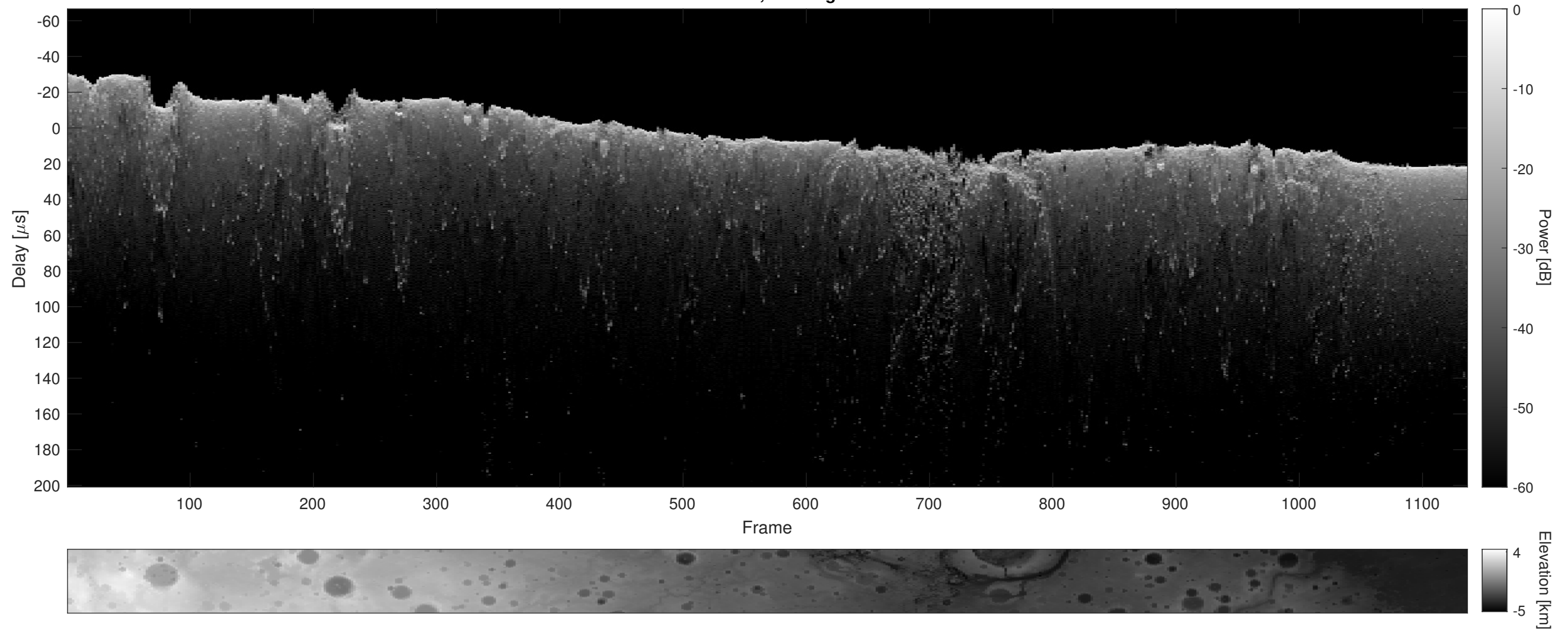
Orbit 20859, Cluttergram
