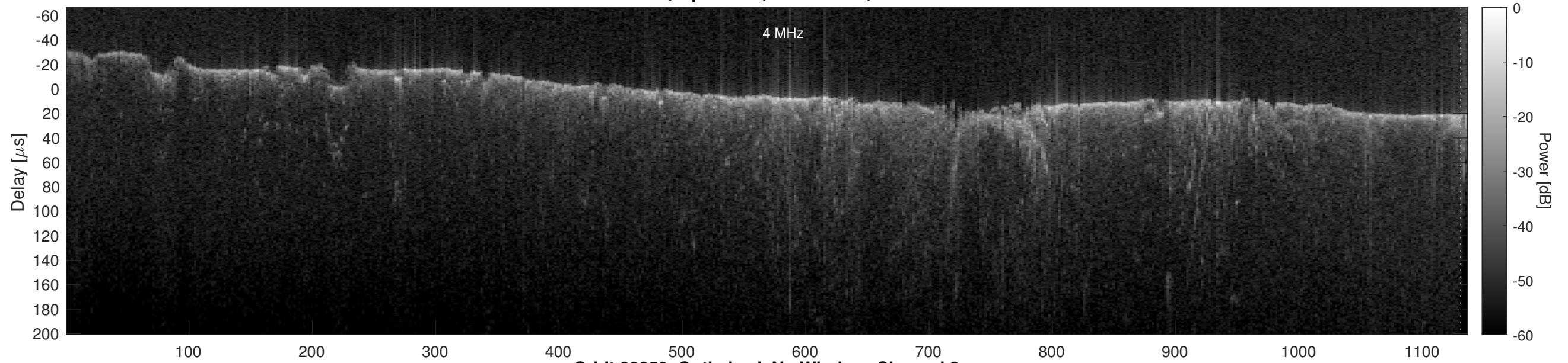
Orbit 20859, Optimized, No Window, Channel 2
