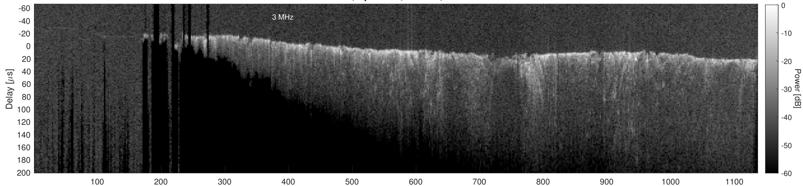
Orbit 20859, Cluttergram
