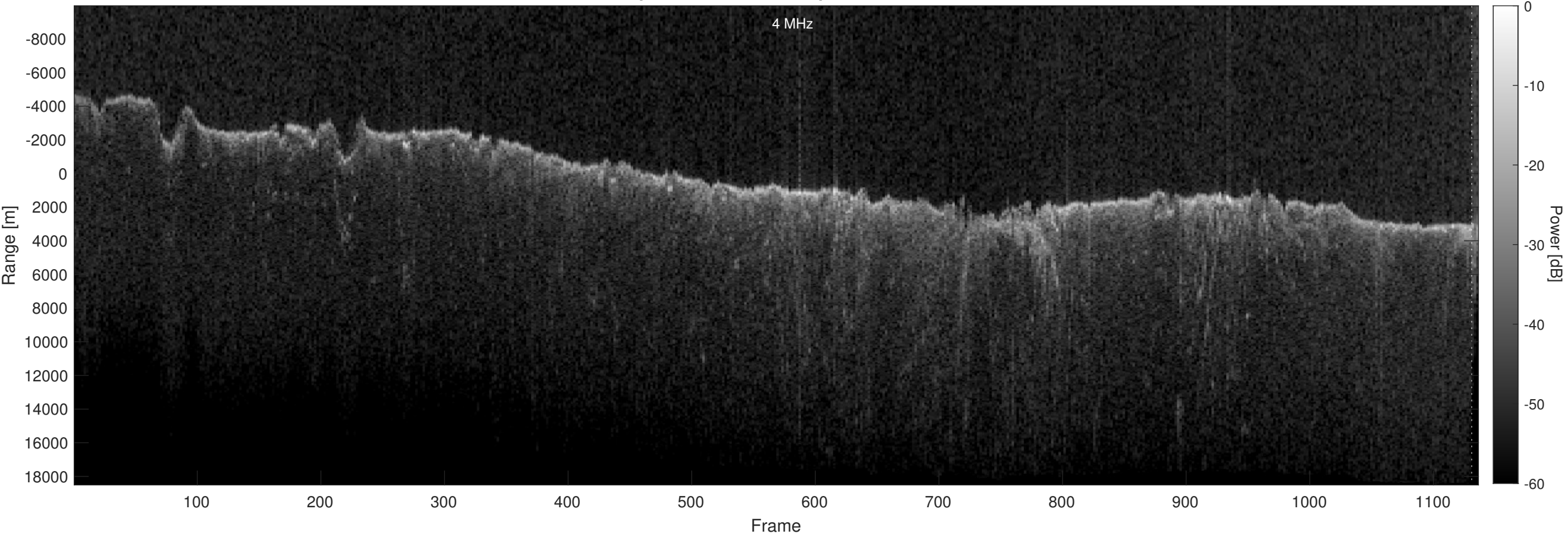
Orbit 20859, Optimized, Window, Depth-Corrected, Channel 2
