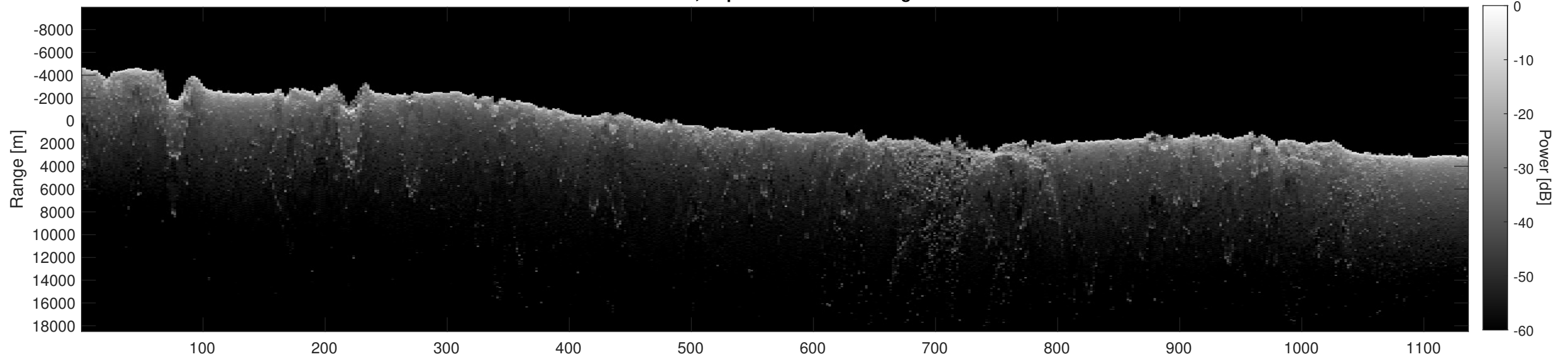
Orbit 20859, Depth-Corrected Cluttergram
