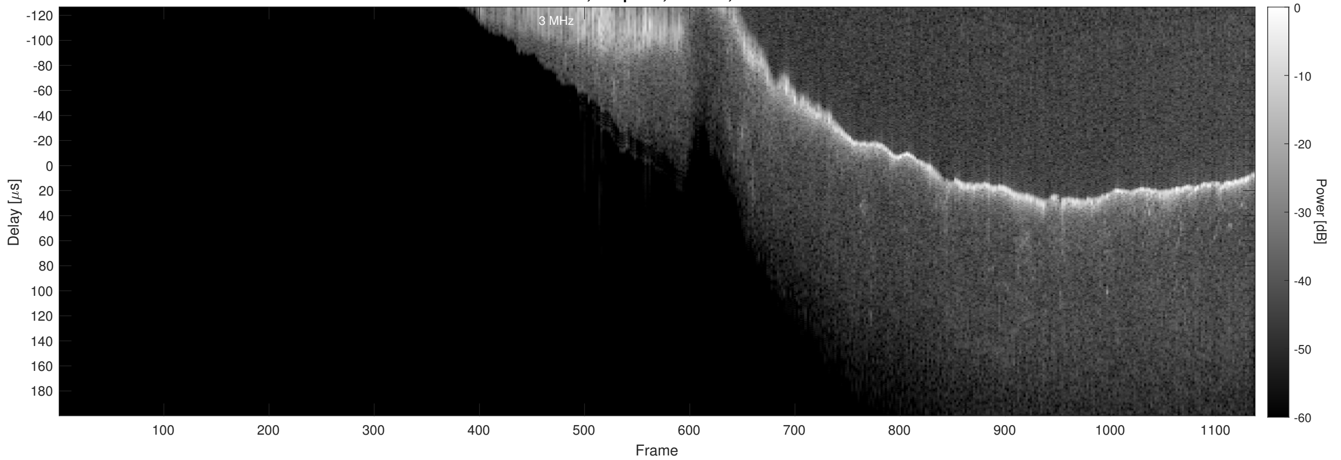
Orbit 20860, Chapman, Window, Channel 2
