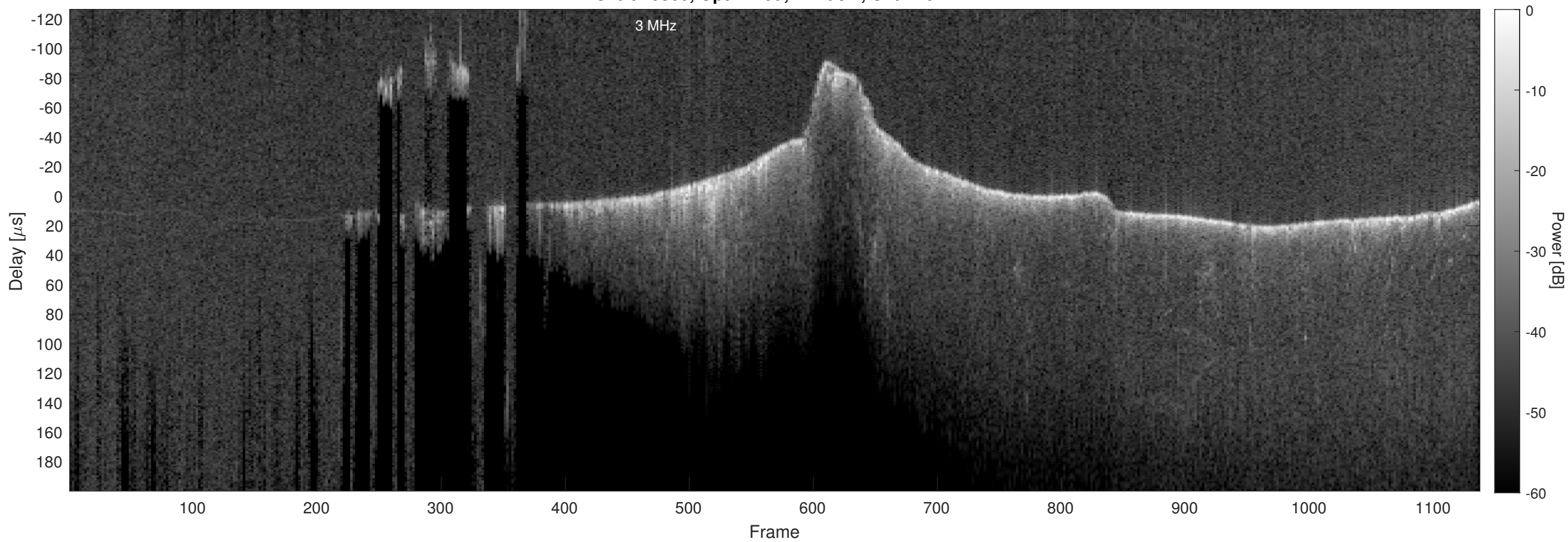
Orbit 20860, Optimized, Window, Channel 2
