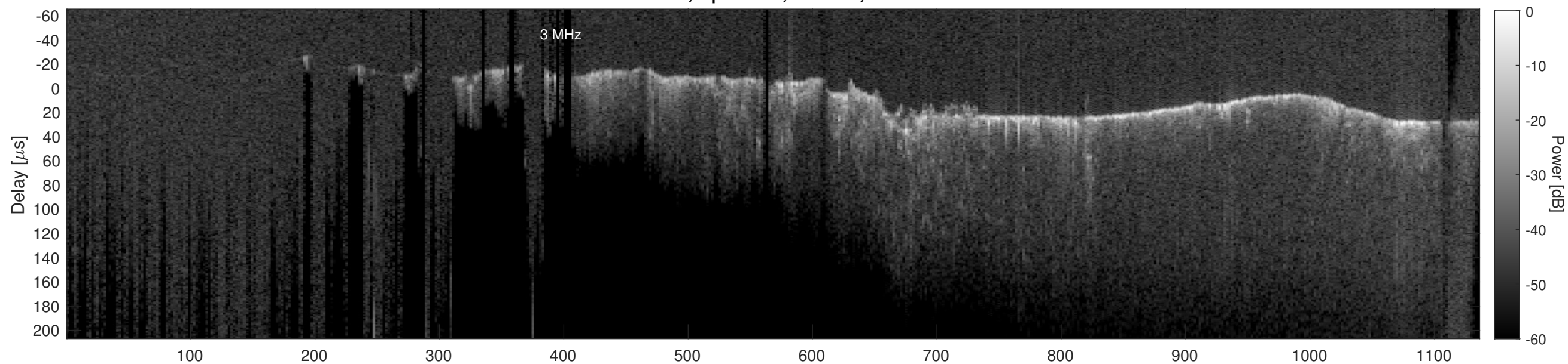
Orbit 20861, Cluttergram
