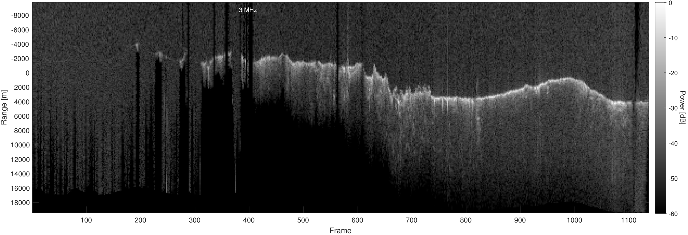
Orbit 20861, Optimized, Window, Depth-Corrected, Channel 2
