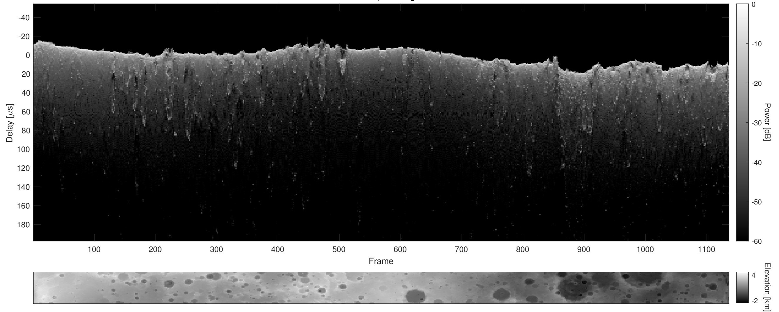
Orbit 20862, Cluttergram
