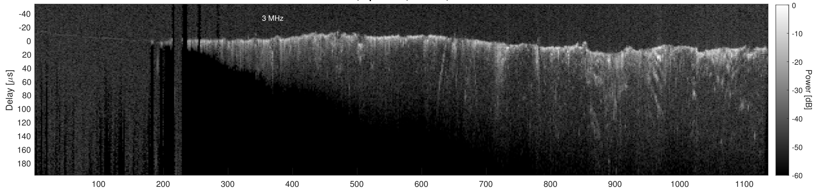
Orbit 20862, Cluttergram
