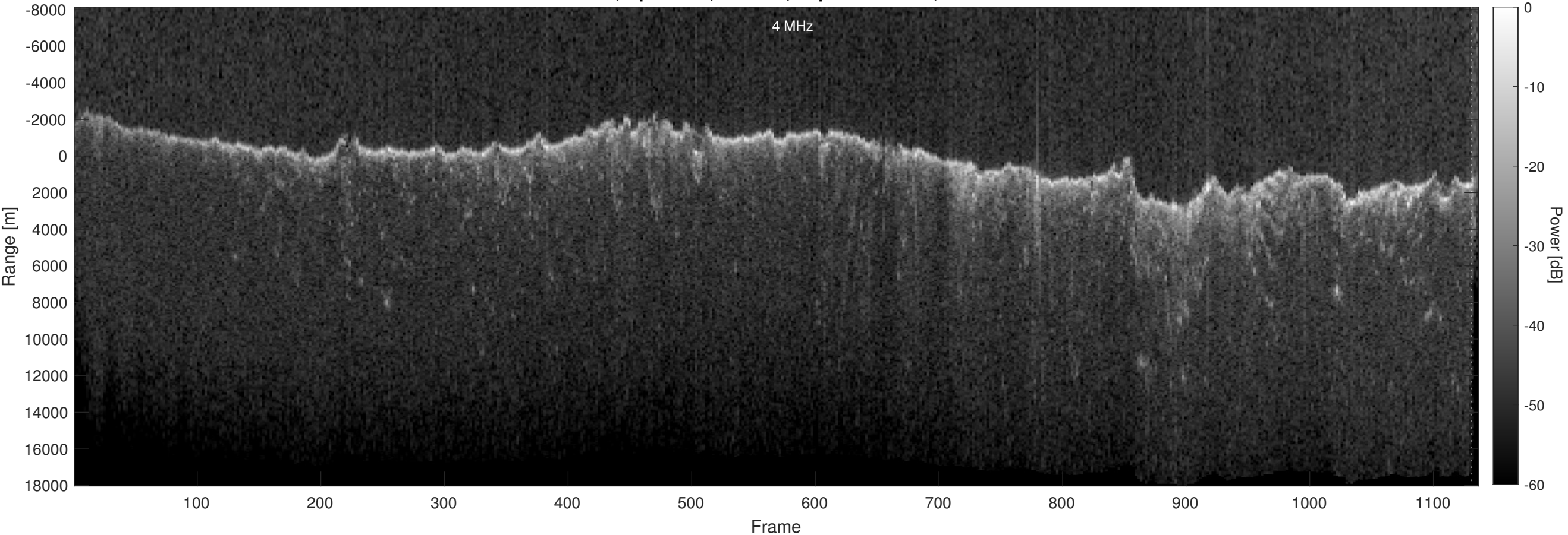
Orbit 20862, Optimized, Window, Depth-Corrected, Channel 2
