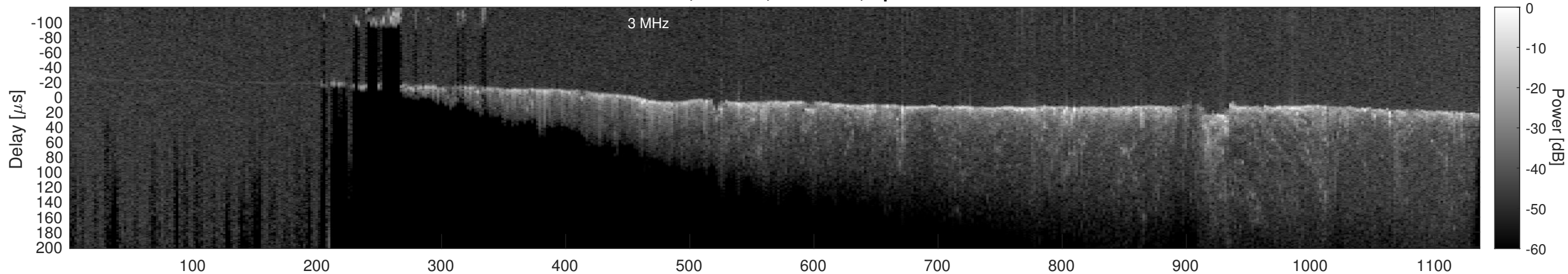
Orbit 20866, Cluttergram
