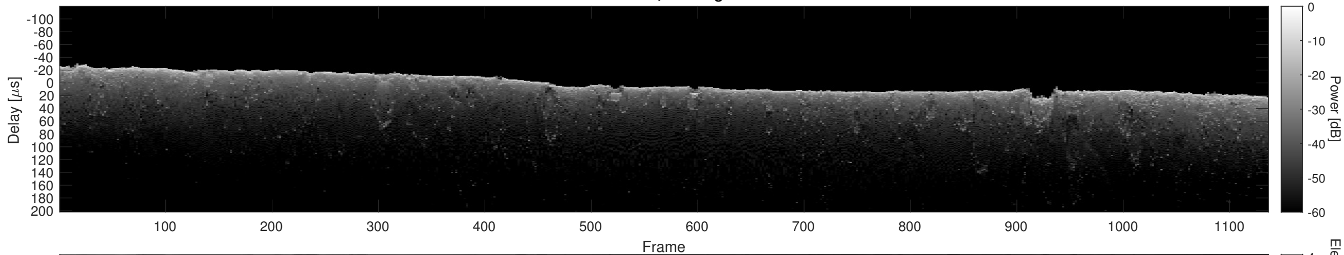
Orbit 20866, Cluttergram
