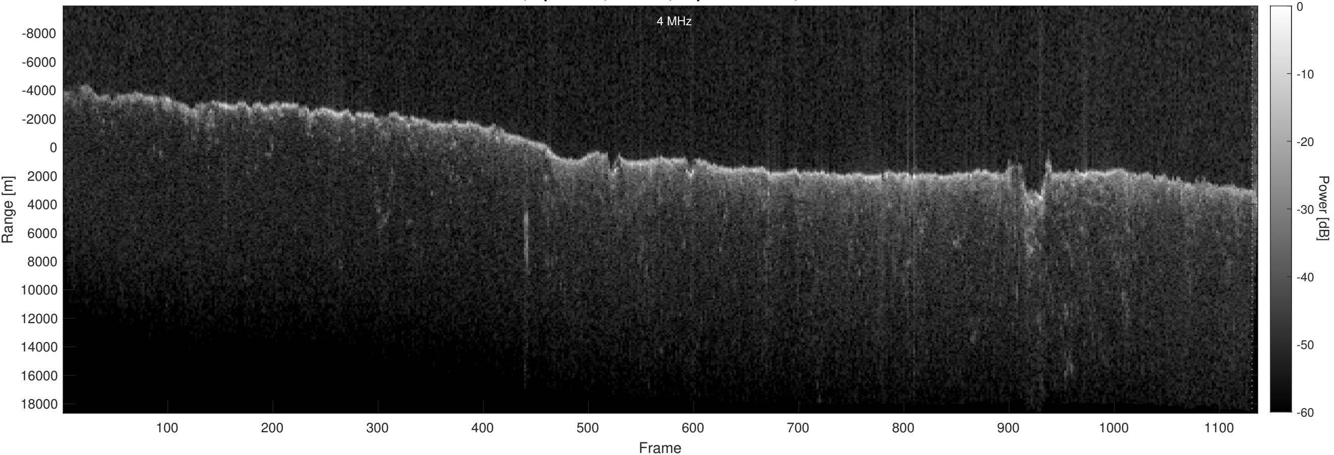
Orbit 20866, Optimized, Window, Depth-Corrected, Channel 2
