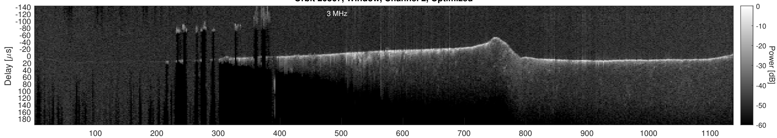
Orbit 20867, Cluttergram
