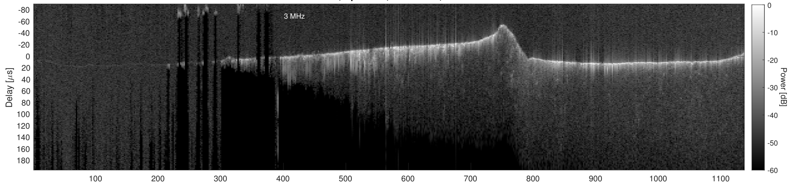
Orbit 20867, Cluttergram
