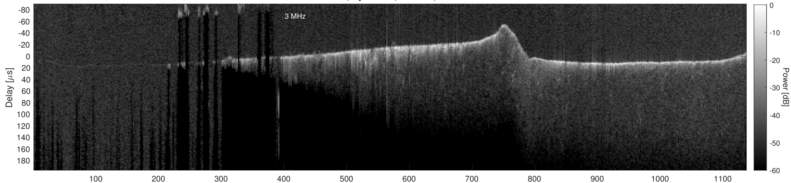
Orbit 20867, Cluttergram
