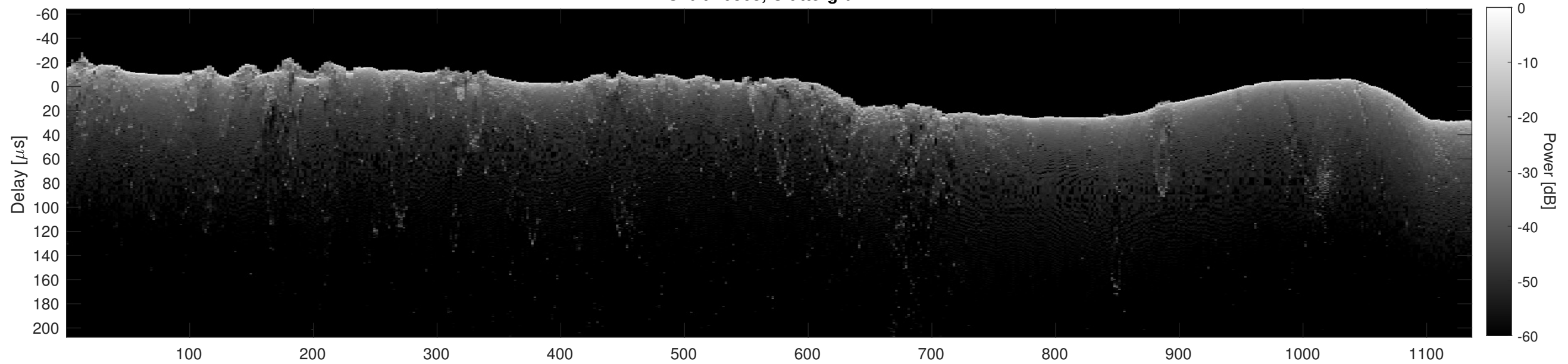
Orbit 20868, Cluttergram
