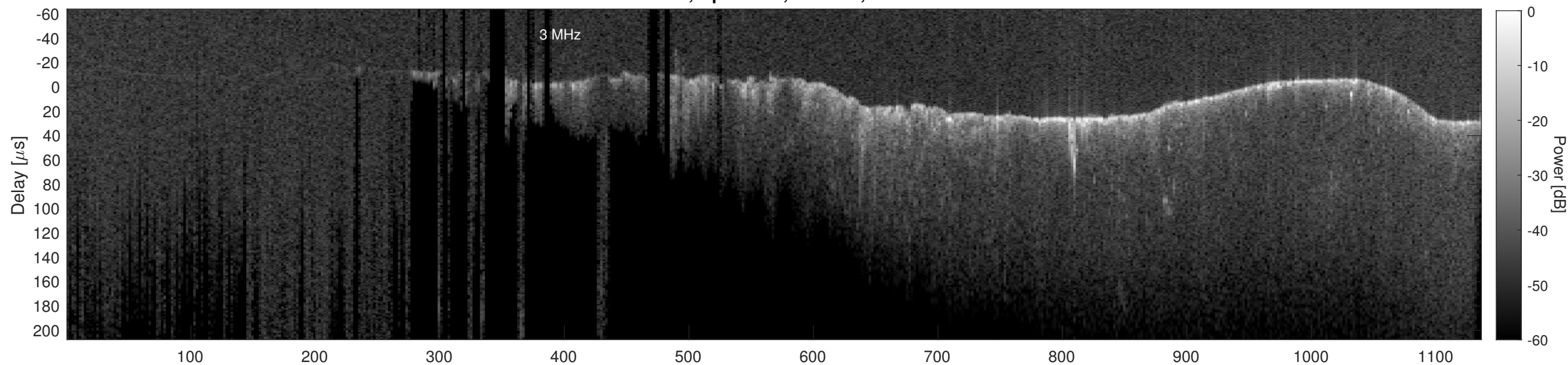
Orbit 20868, Cluttergram
