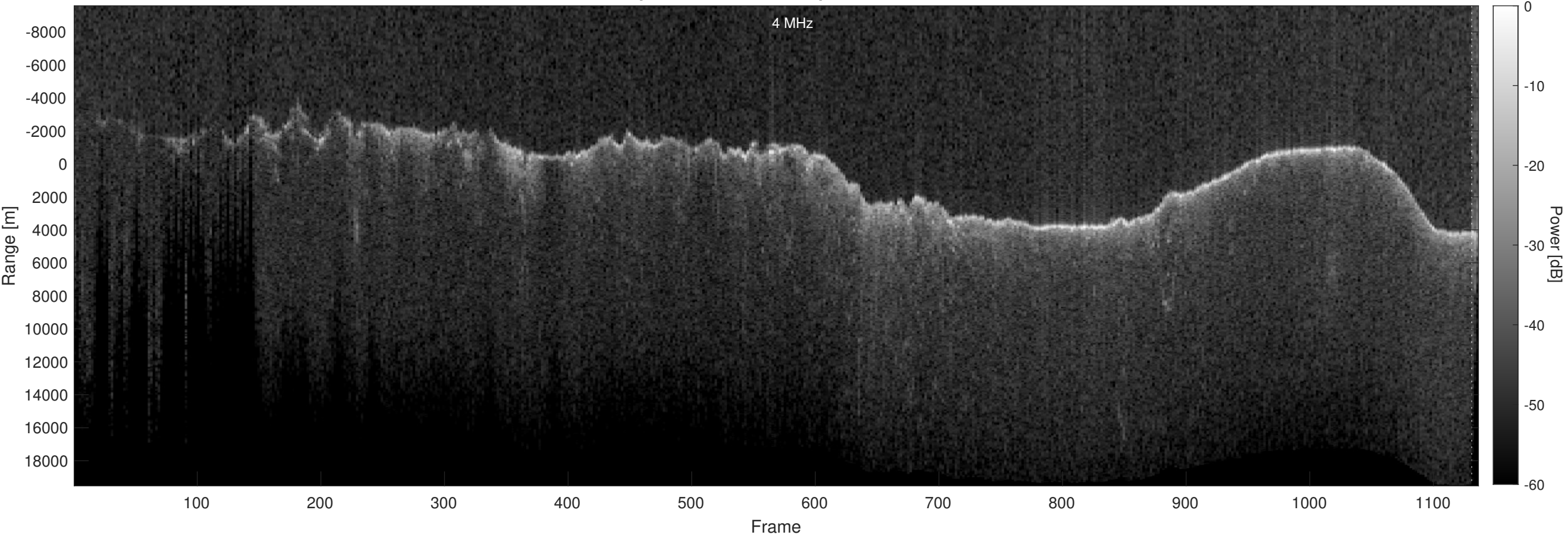
Orbit 20868, Optimized, Window, Depth-Corrected, Channel 2
