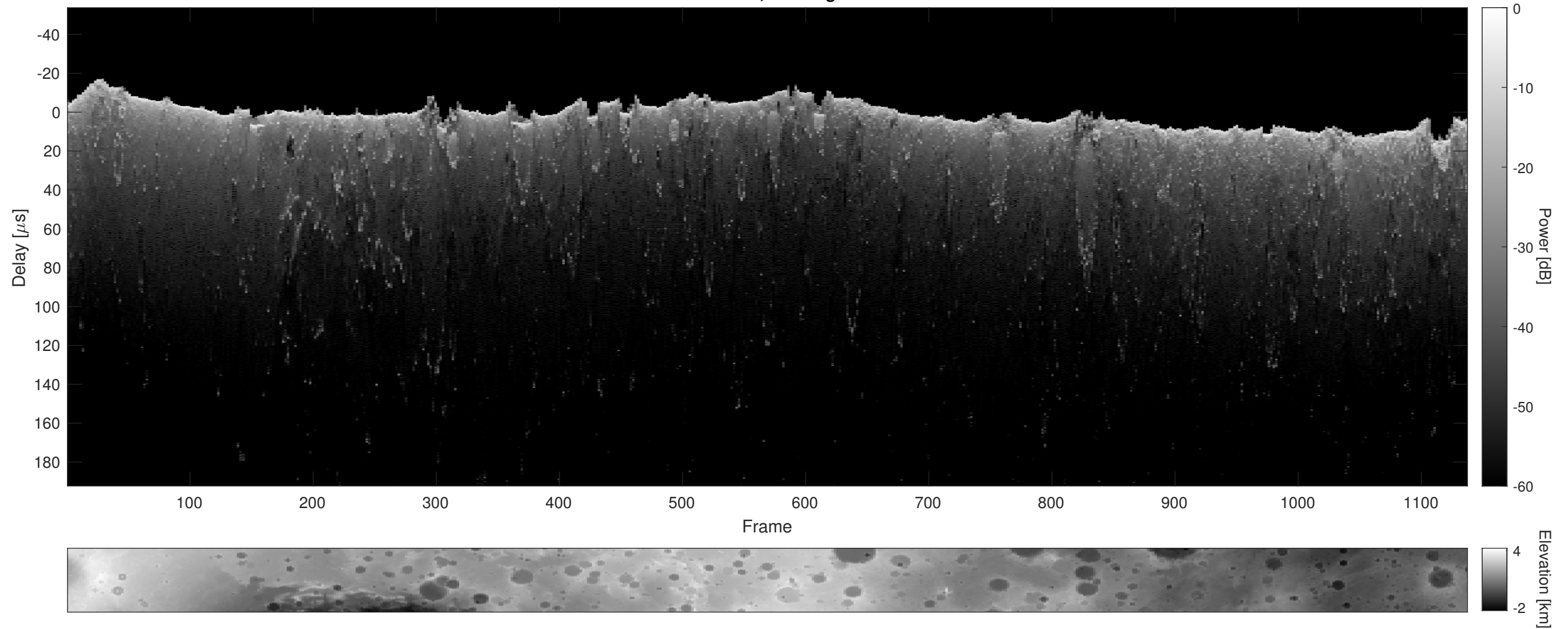
Orbit 20869, Cluttergram
