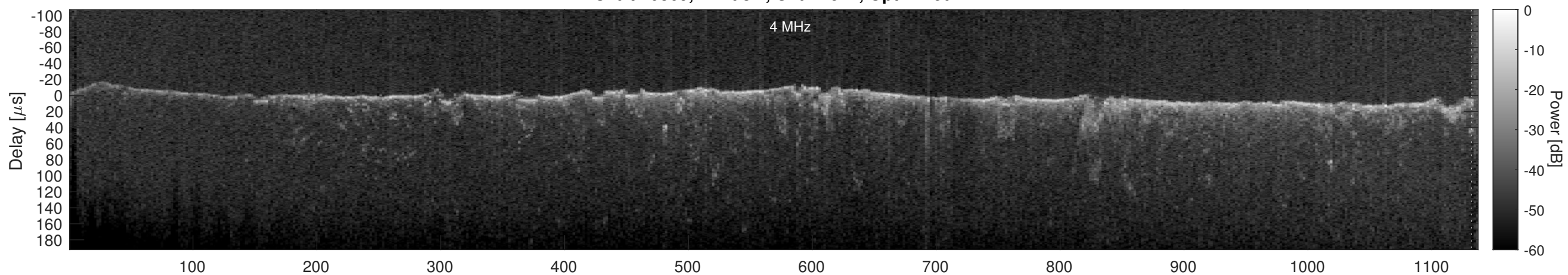
Orbit 20869, Cluttergram
